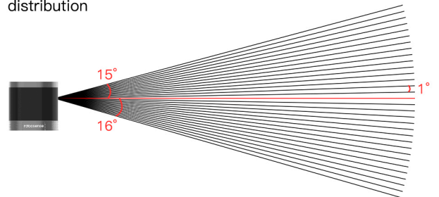
Helios 32: 31° Vertical FOV, 32-Beam even distribution
